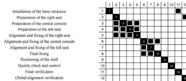
Figure 19. Design Structure Matrix (DSM) of the traditional process using OBDC method
