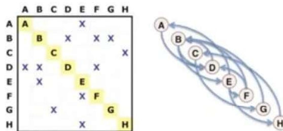
Figure 1. biunivocal correspondence between DSM matrix and digraph
