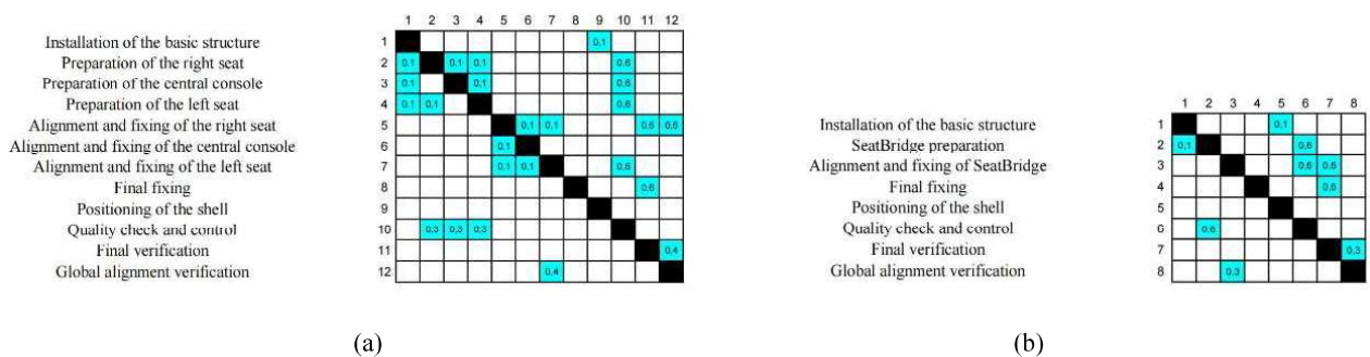
Figure 13. DSM Rework Probabilities of the traditional process (a) and the innovative process (b)
